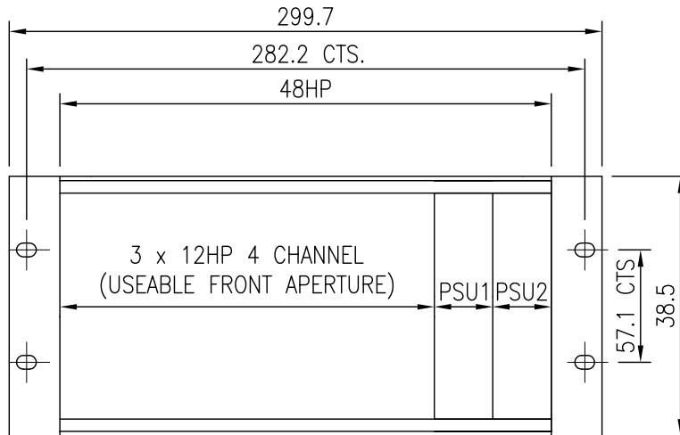
FRONT OF THE RACK
